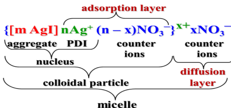
Figure 4 – The formula of the silver iodide micelle stabilized with silver nitrate
