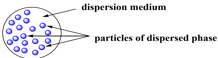
Figure 1 – A model of a dispersed system
